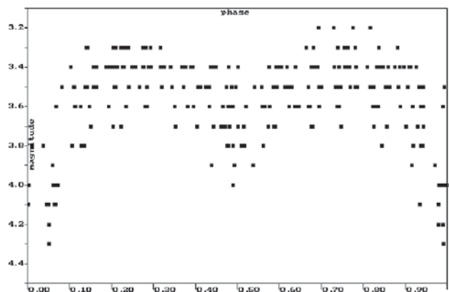
Figure 10. Light curve of \beta Lyrae for 1998 (SAC 65 elements.)
