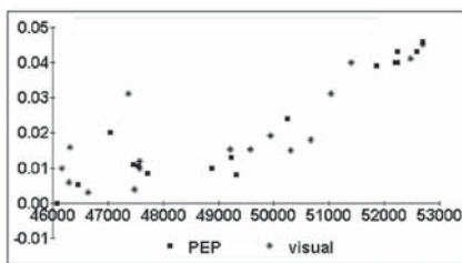
Figure 9. O-C (Observed-Computed) diagram for RZ Cas since the mid-1980s, showing the evolution of the discrepancy with time.
