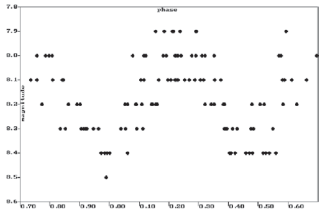
Figure 3. Light curve of W UMa in 1996–1999, from observations by the author.
