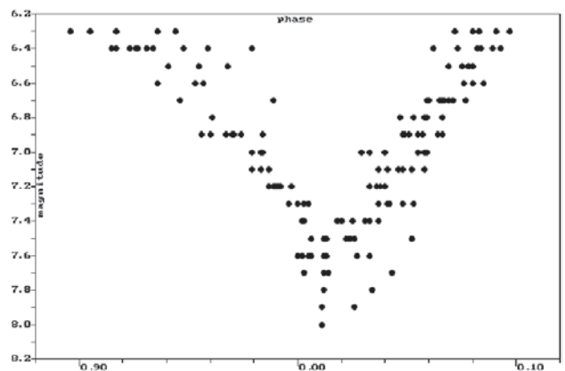
Figure 4. A primary eclipse of RZ Cassiopeiae in 1993. Note the sharp V-shape of the light curve.
