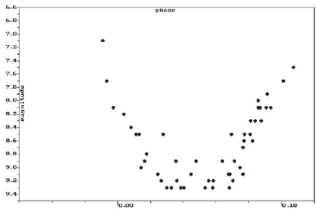
Figure 6. Eclipse of U Cep in 1999 (GCVS elements).
