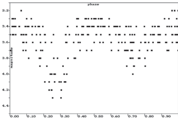
Figure 2. Light curve of \beta Lyrae over a 13-day orbital period in 1998.
