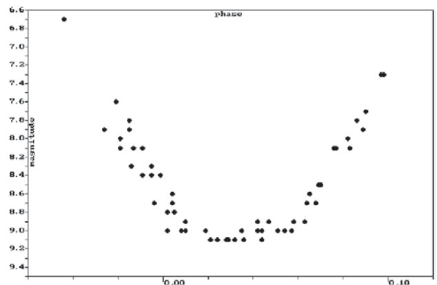
Figure 5. The U-shaped eclipse of U Cephei in 1996 (GCVS elements).
