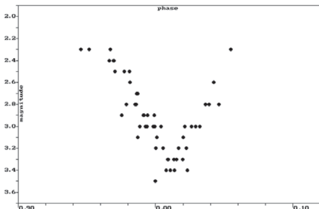
Figure 1. The eclipse of Algol in 1999, using GCVS elements.
