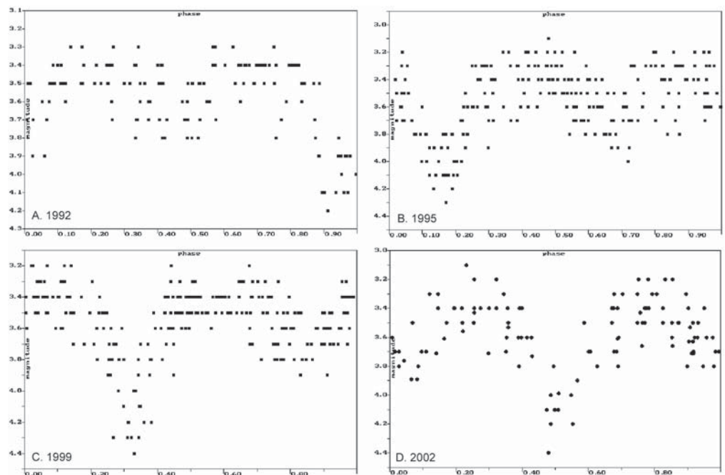
Figure 7. Observations of \beta Lyrae in 1992, 1995, 1999 and 2002 (GCVS elements).
