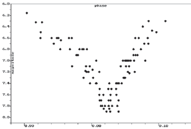
Figure 8. Lightcurve of RZ Cas in 1999 (GCVS elements).
